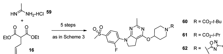
Scheme 8. Preparation of C2-Methyl Analogues 60–62
